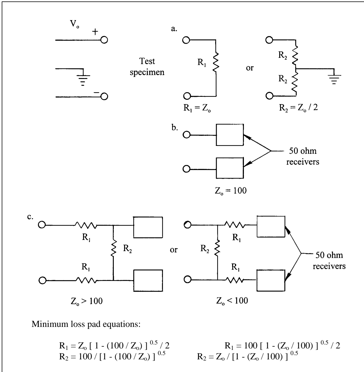
Figure E.2 - Differential (balanced) terminations
