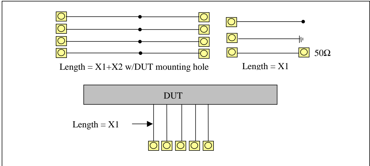
Figure C.1 – Typical mother board test fixture
