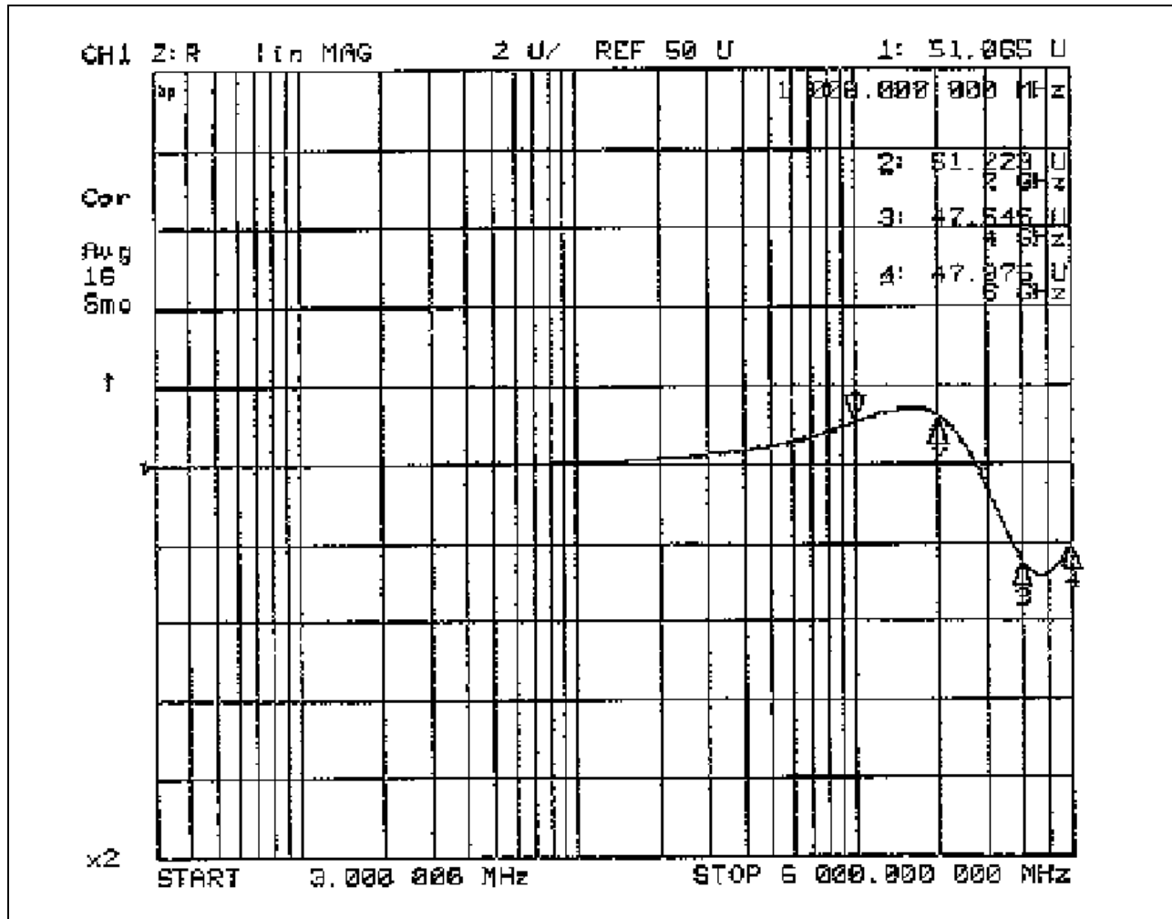
Figure A.3 – Example of analyzer output, impedance vs. log frequency plot
