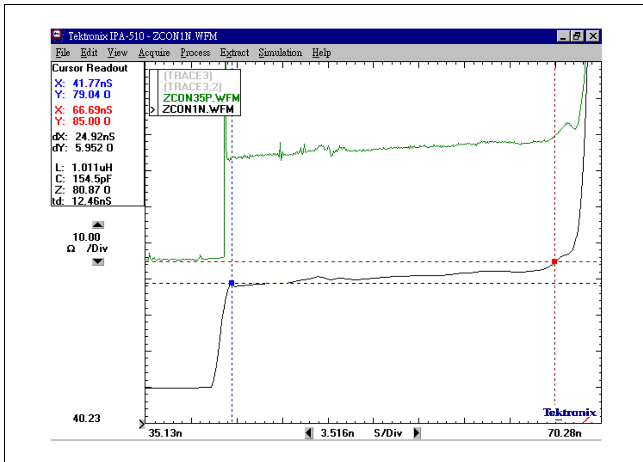
Figure D.2 – Example of impedance profiles of cable under the rise time of 35 ps and 1 ns
