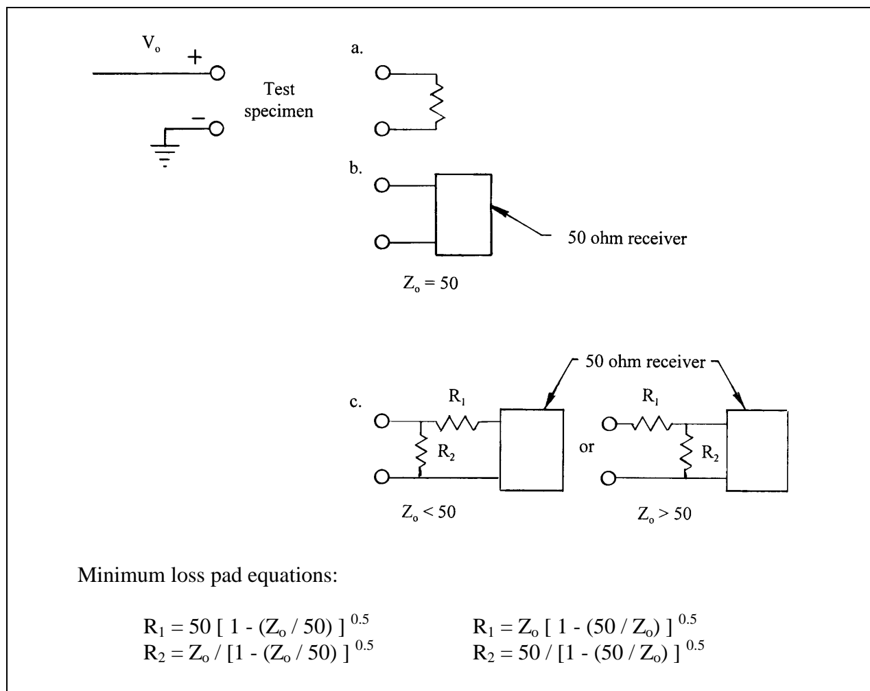
Figure E.1 - Single-ended terminations
