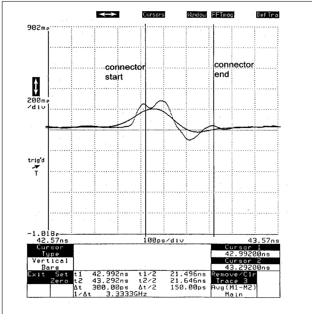
Figure A.2 – Example of TDR output; 2 curves (different rise times) and start and stop specimen points
