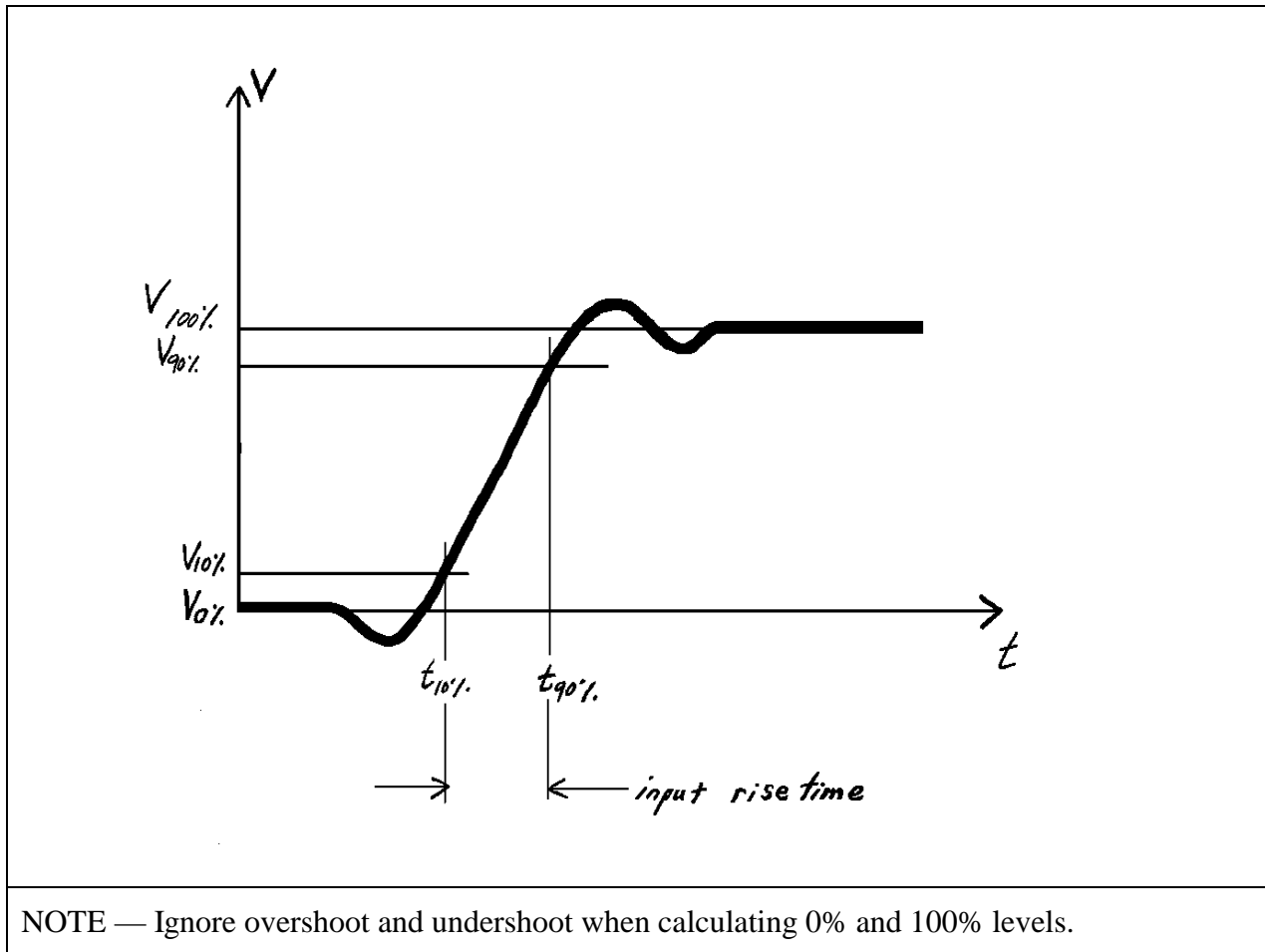
Figure A.1 – Example of rise time measurement points
