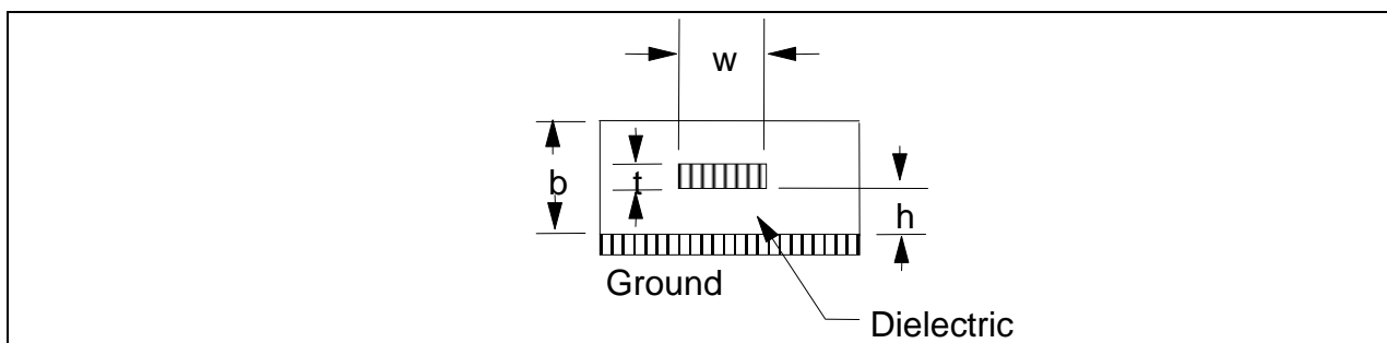
Figure G.2 - Buried microstrip geometry
