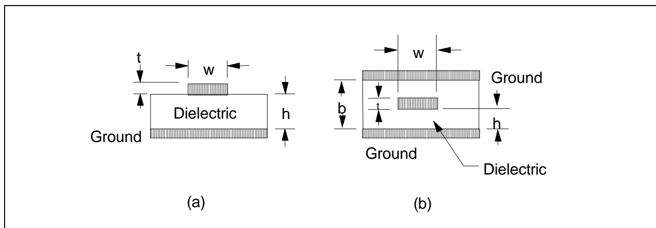
Figure G.1 - Microstrip (a) and stripline (b) geometries
