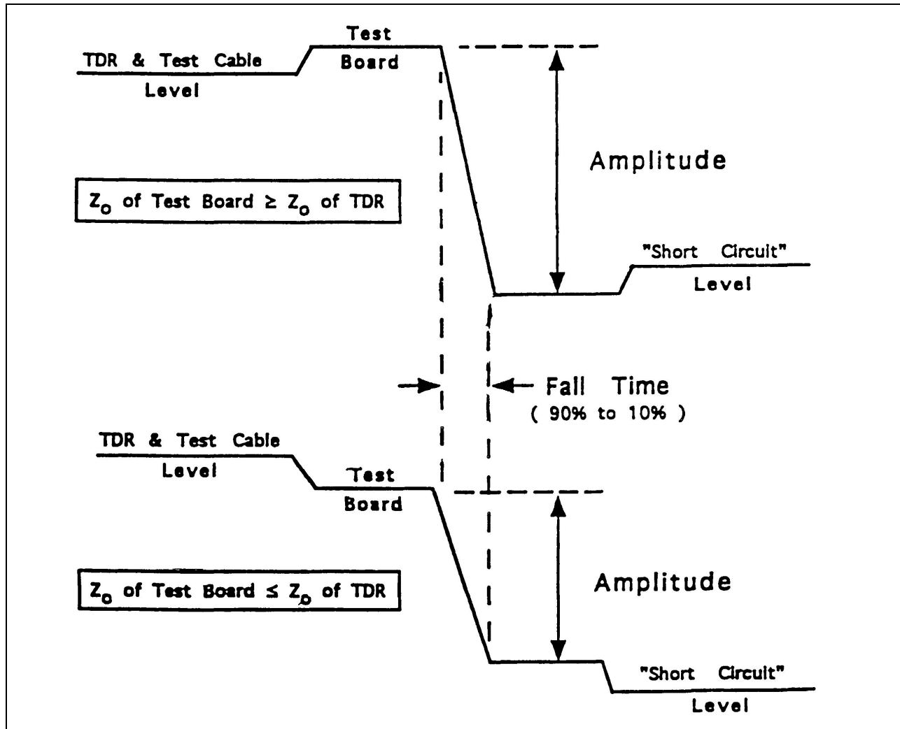
Figure C.3 – Example of near end reference trace
